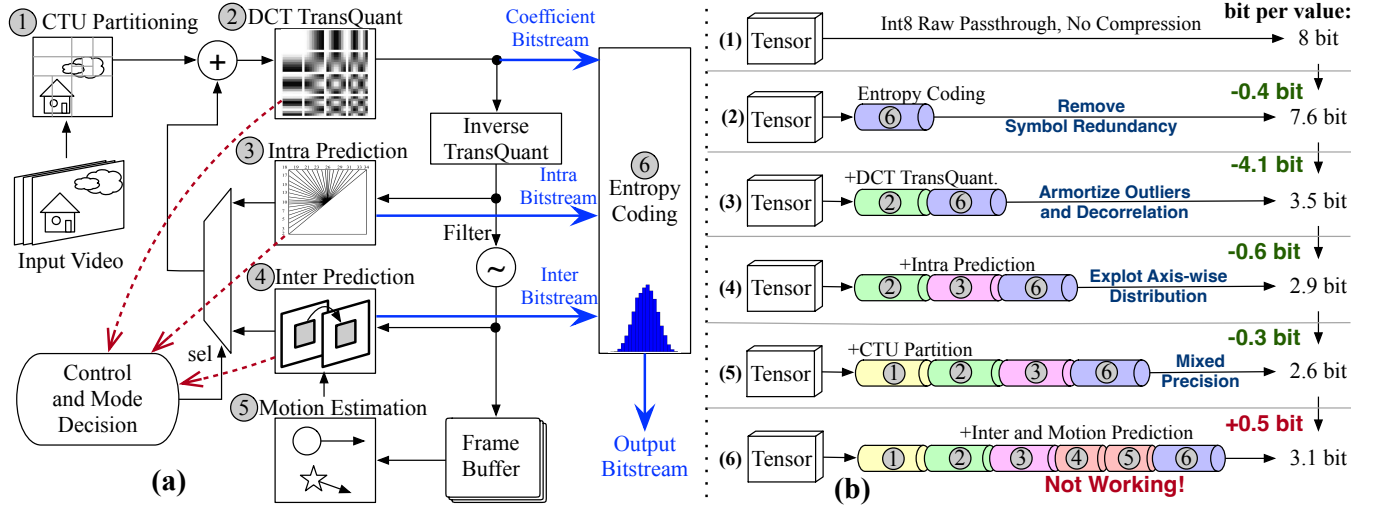
Figure 2: Why does the Video Codec Work for LLM? (a) illustrates the pipeline of the H.265 video encoder. In (b), we incrementally activate the stages in the H.265 video encoding pipeline to demonstrate how each step contributes to the compression process. We constrain the quality of the compression/decompression process to have a maximum mean square error of 0.01.
